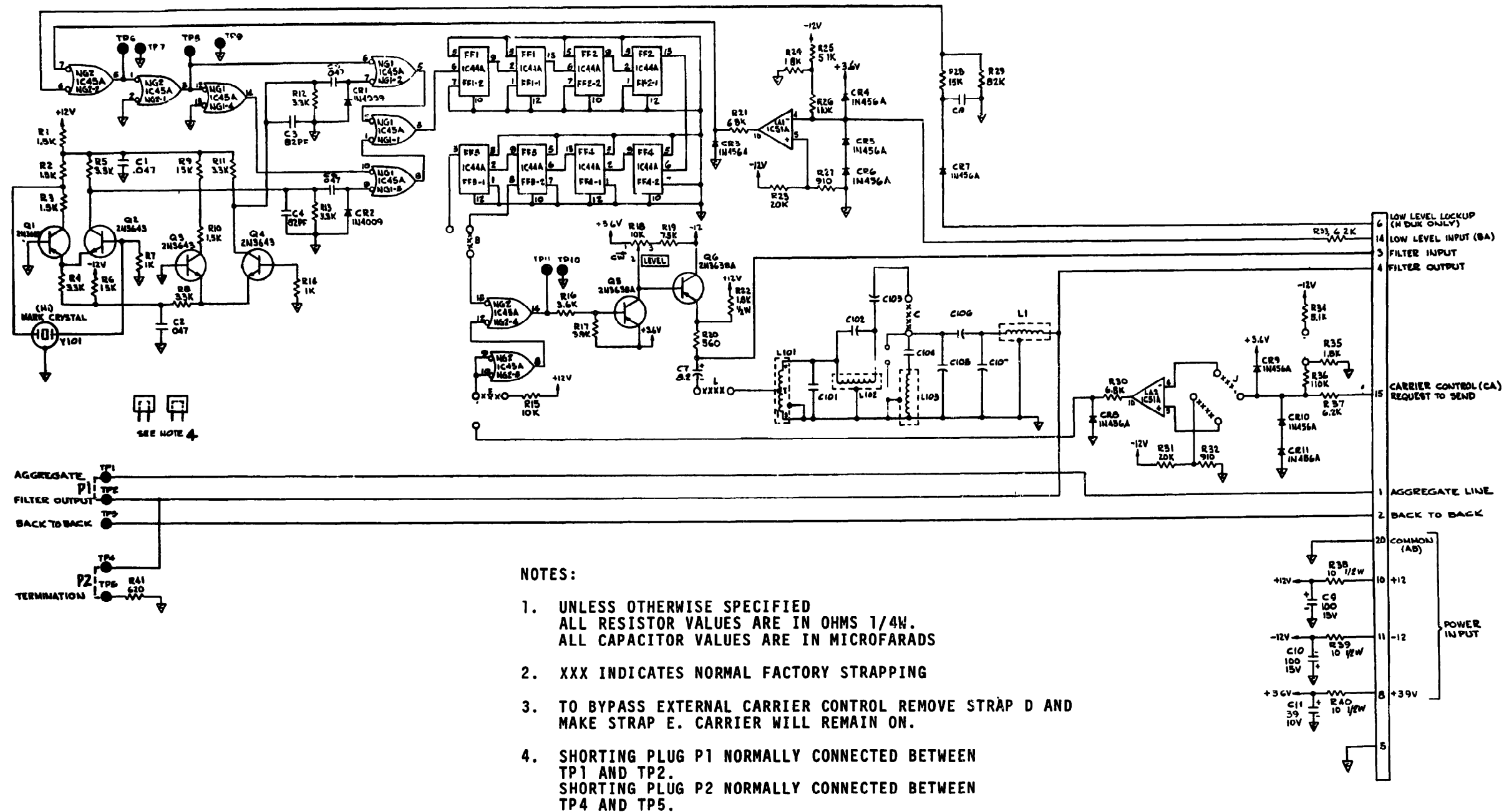
Figure 7. Keyer 70795, Schematic
